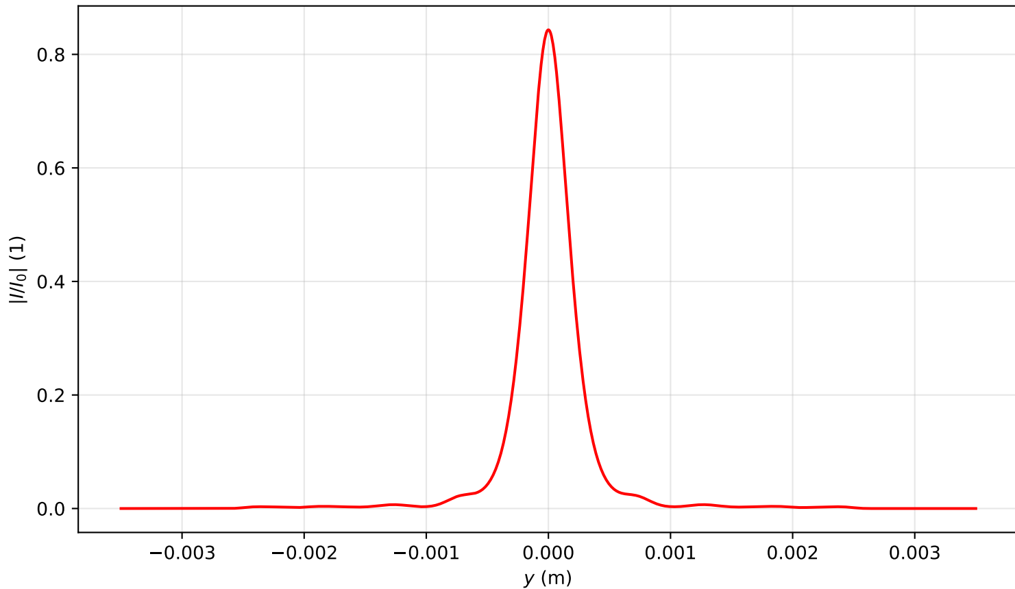
Intensity profile I(x = 0, y, z = 3.662)/I_0 , \text{Pin}=3.0\text{Pcr} , artificial time
